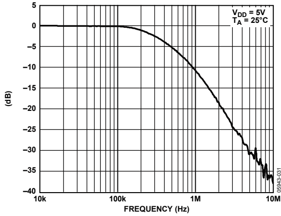
Figure 29. Multiplying Bandwidth
