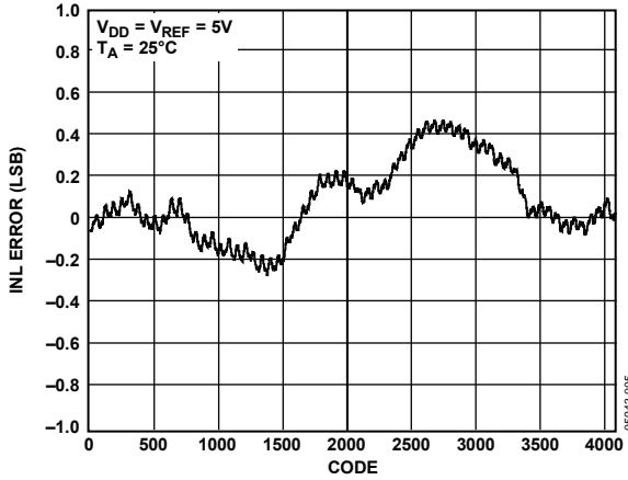
Figure 6. INL AD5624
