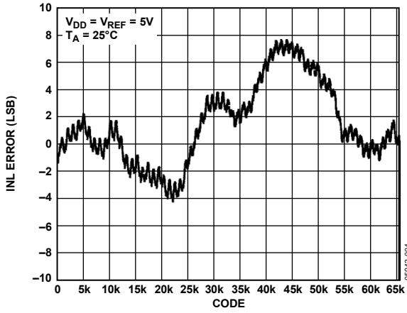
Figure 5. INL AD5664
