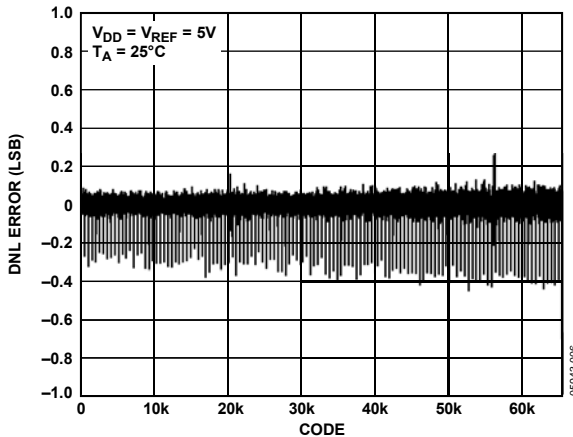
Figure 7. DNL AD5664
